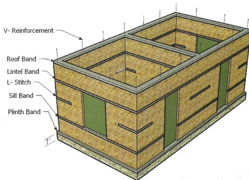
Brick house reinforced with steel rods for extra strength
